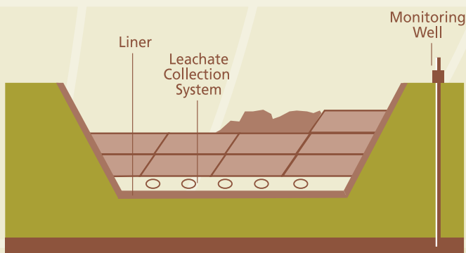
Figure 1—Cross-Section of a Typical, Properly Designed, Constructed, and Maintained Landfill
