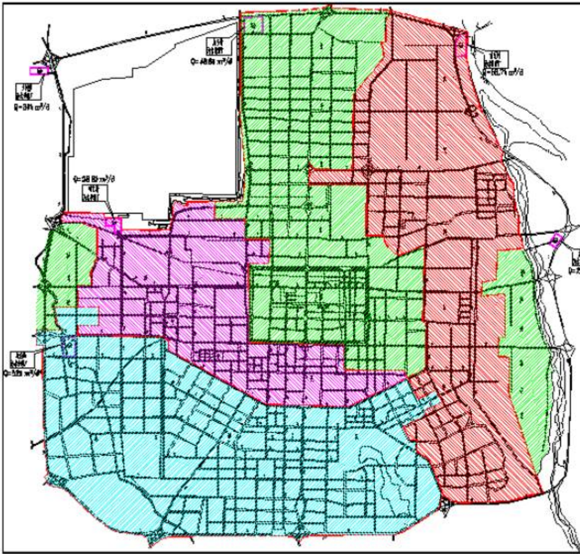
Sewer System and Service areas in Xi'an
